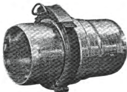
Complete assembly, female press-in coupler half, male press-in coupler half, gasket and band assembly. Used for main-line installation. Galvanized. Hold bands recommended for installing to aluminum tubing.
